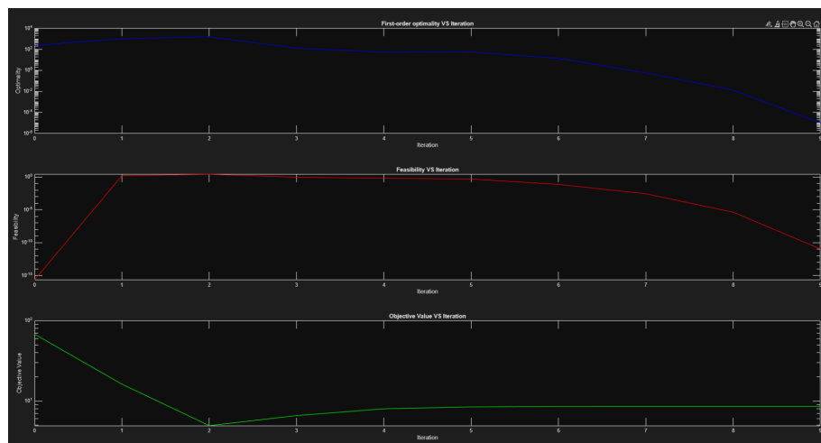
Figure 7 - Optimization convergence study
