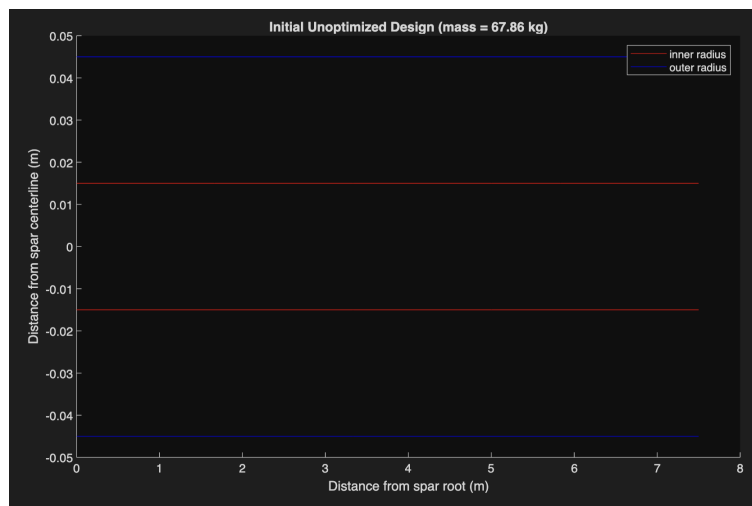
Figure 5 - Initial spar design geometry before optimization
