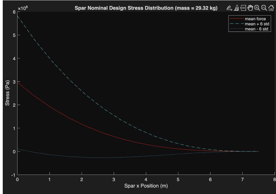
Figure 4 - Nominal spar design stress distribution
