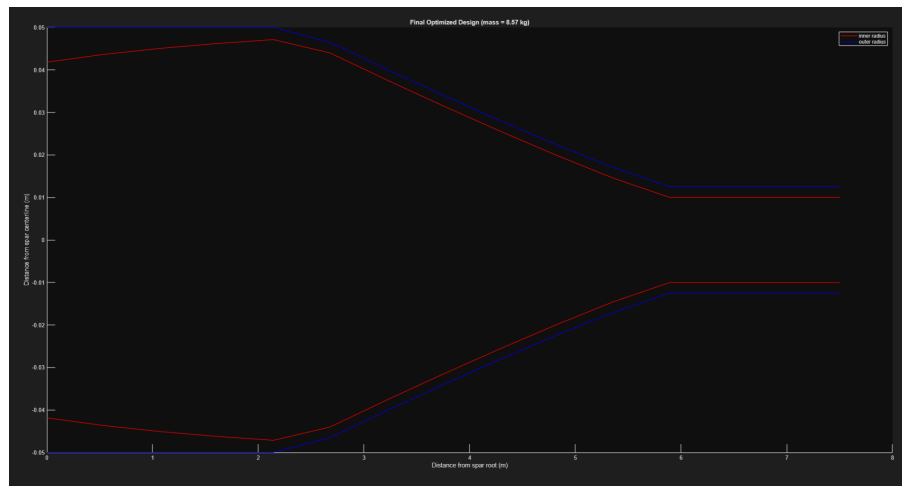
Figure 6 - Optimized spar design geometry
